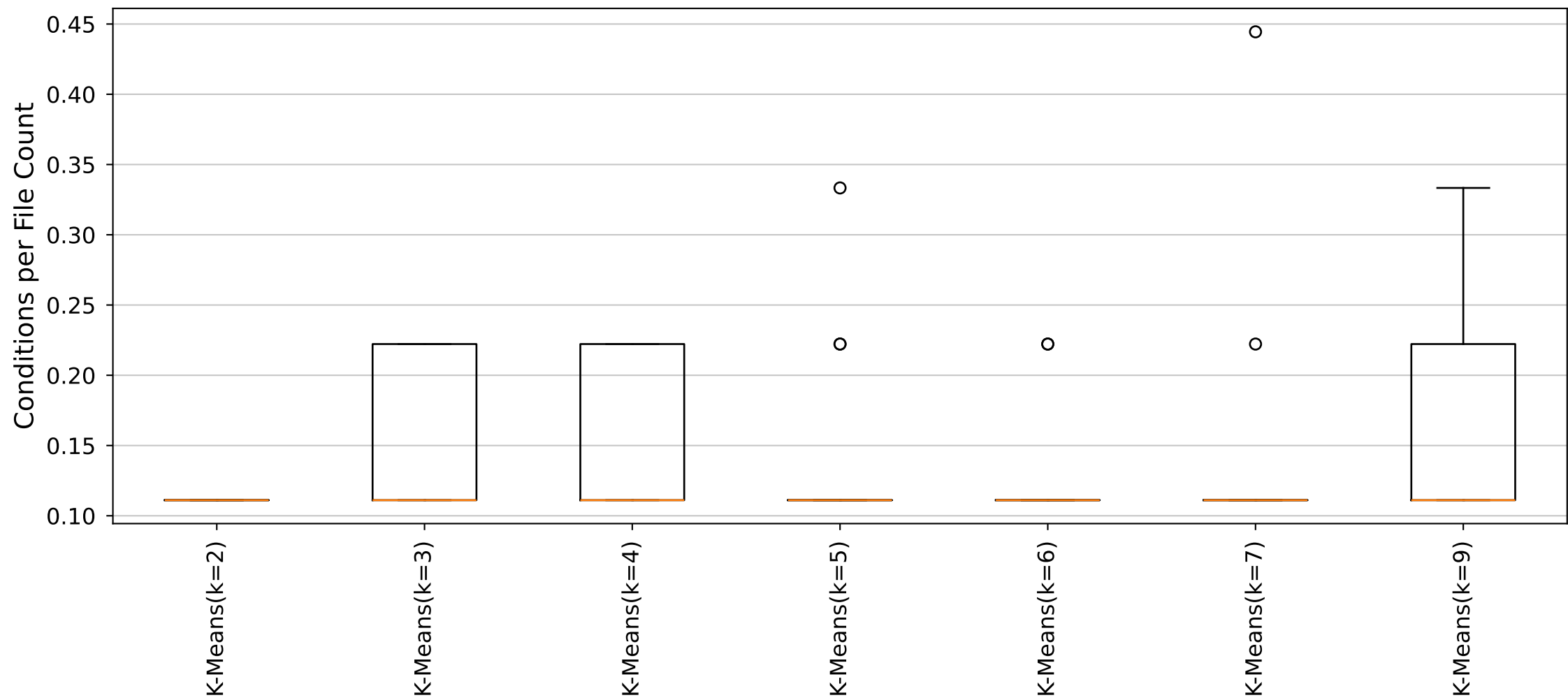
YARA Rules Conditions per File Count Distribution (Cluster12_Size9 dataset)
